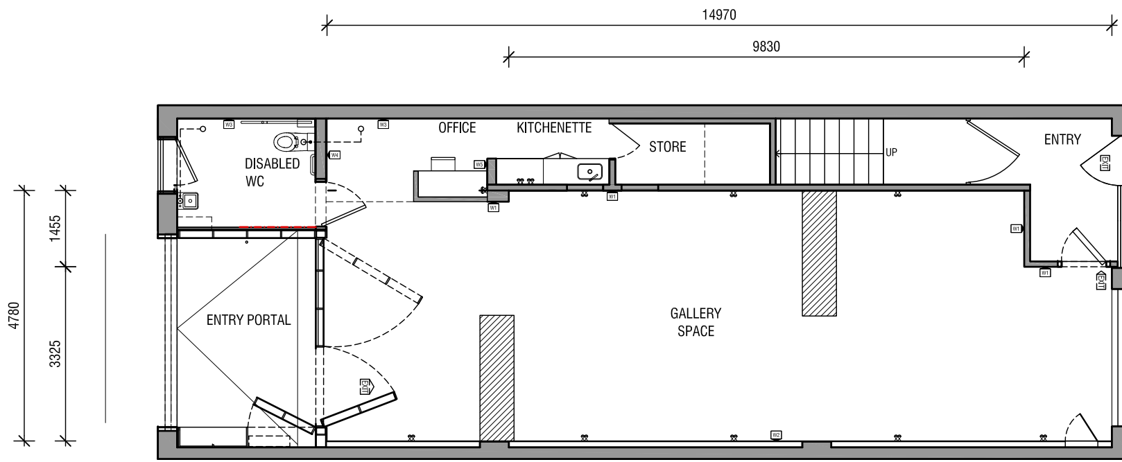
GLASSHOUSE GALLERY PLAN 1:100@A4
